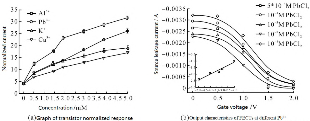
Figure 7. Sensing performance of FEETs sensor.
