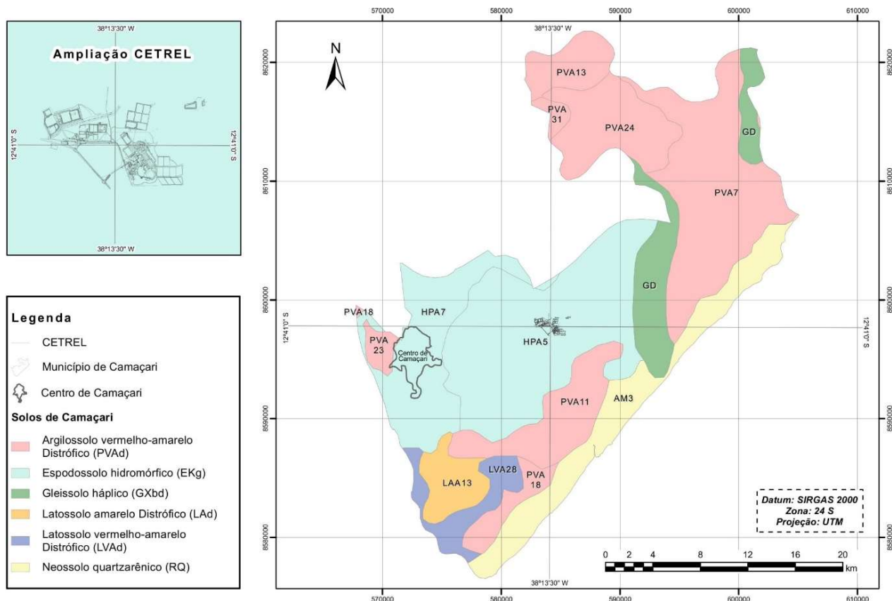
Figure 6. Pedological map of the municipality of Camaçari and the CETREL region. Source: Adapted from CPRM [35].
