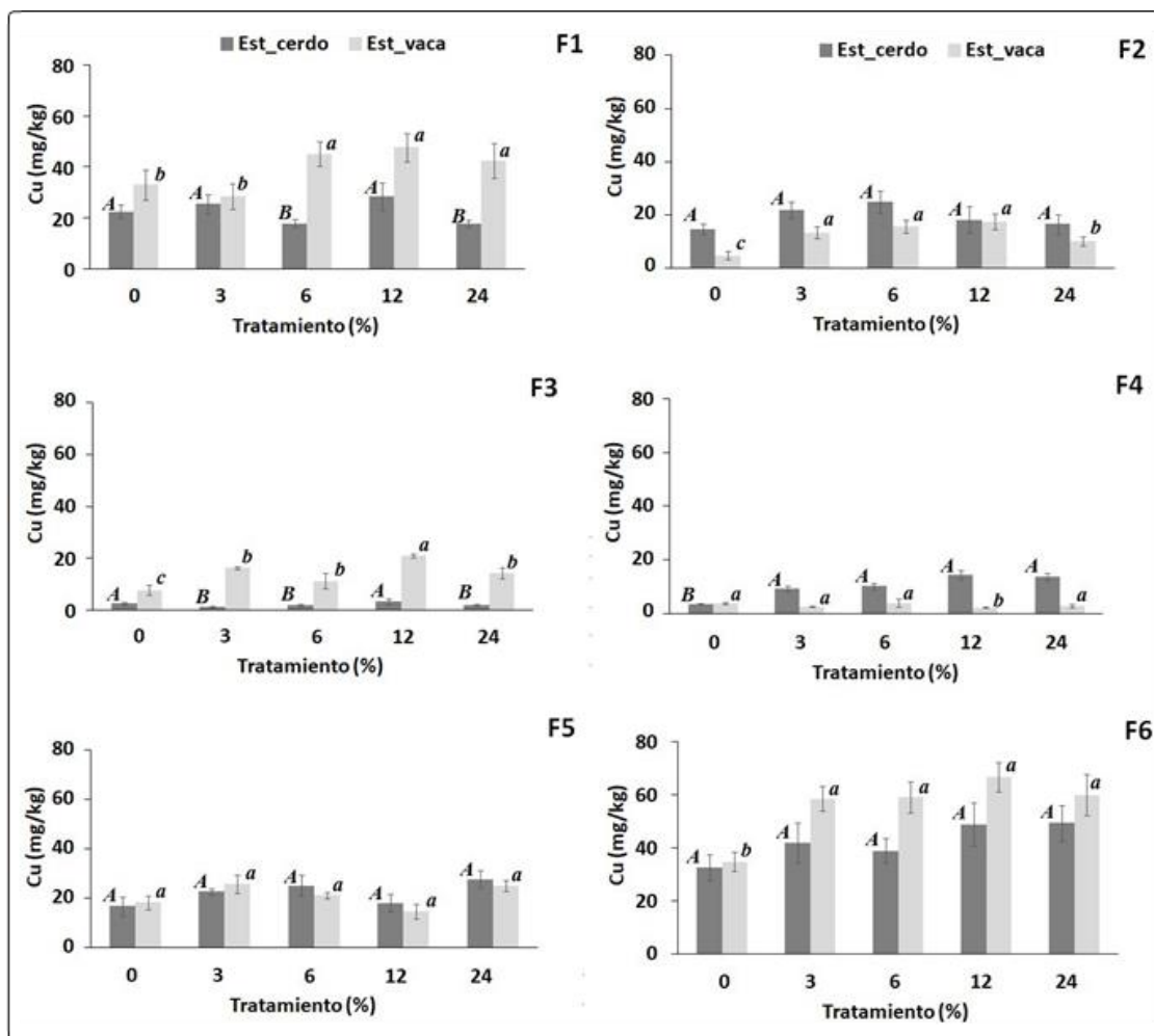
Figure 1. Chemical fractions of Cu in pig and cow manure treatments; F1 = Cu-soluble-exchangeable, F2 = Cu-bound to Fe and Mn oxides, F3= Cu-bound weakly to OM, F4 = Cu-bound strongly to OM, F5 = Cu-bound to sulfide phase and F6 = Cu-bound to residual solid. Treatments with the same letter in each graph are not significantly different (Tukey test: \alpha = 0.05 ). Personal elaboration
