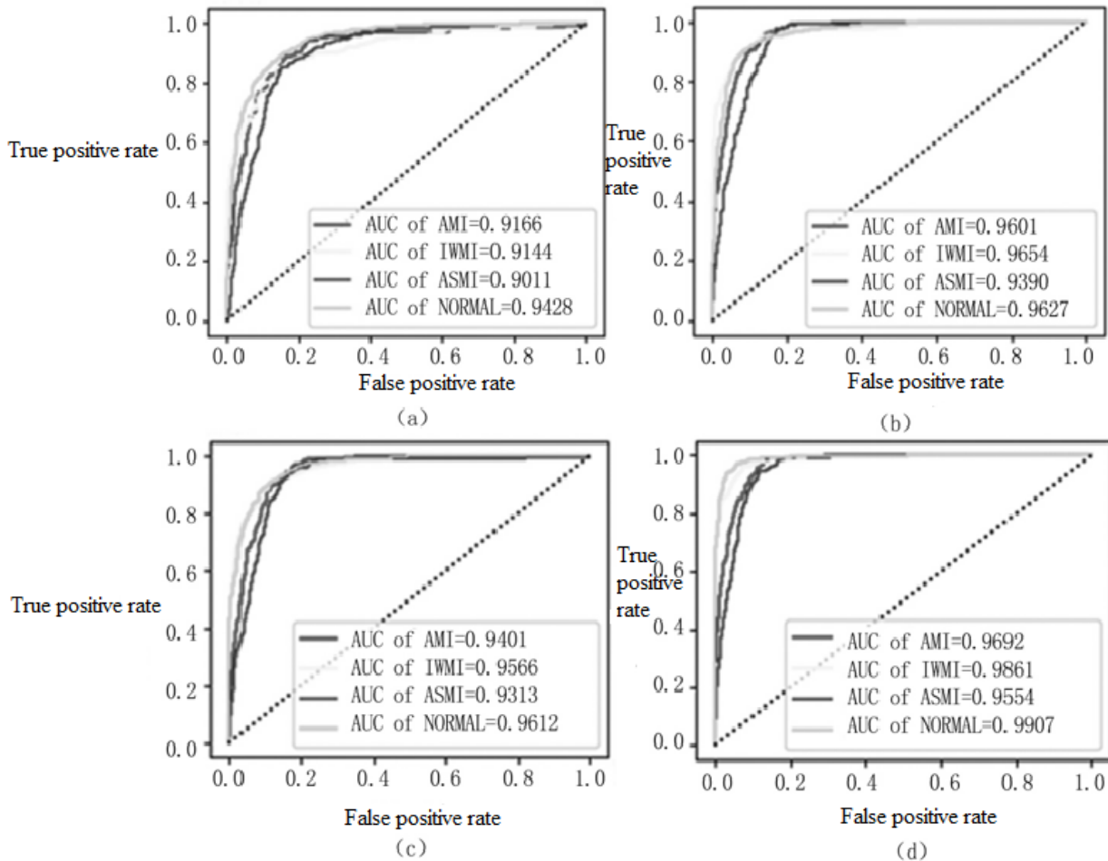
Figure 6. Comparison of Multi resolutionresnet and classic CNN's ROC curve on train data (a) Lenet; (b) VGG; (c) Resnet34; (d) Multi resolutionresnet.
