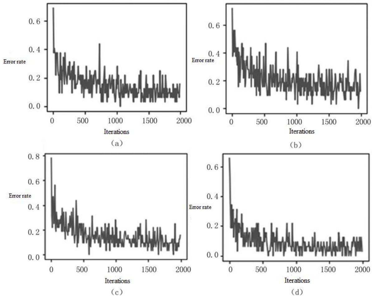
Figure 5. Comparison of Multi resolutionresnet and classic CNN's convergent curve on train data (a) Lenet; (b) VGG; (c) Resnet34; (d) Multi resolutionresnet.
