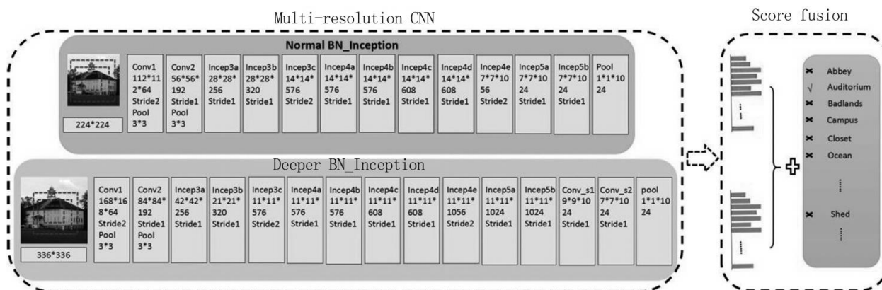
Figure 2. Multi resolution CNN.
