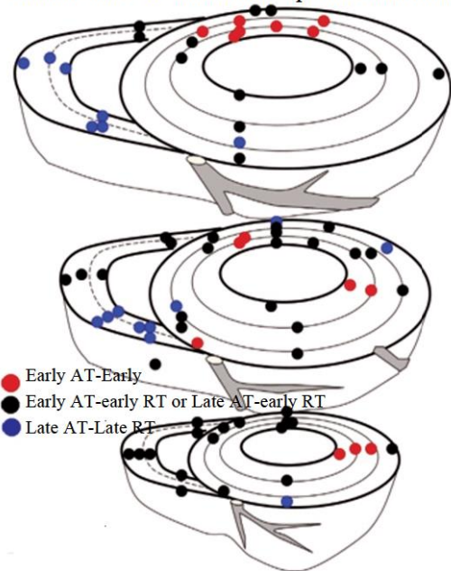
The heart was perfused by Langendorff in vitro with a pacing interval of 700ms. Black represents the sites whose depolarization time is earlier than the median time of depolarization and whose repolarization time is later than the median time of repolarization, or the sites whose depolarization time is later but whose repolarization time is earlier. Red represents sites with early depolarization and early repolarization. Blue represents sites with late depolarization time and late repolarization time[30]
