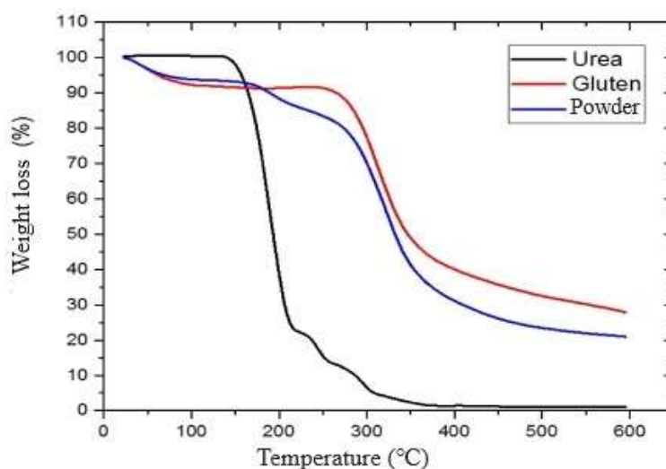
Figure 3. Thermogravimetric analysis (TGA) of the evaluated materials: (a) urea, (b) gluten powder and (c) SLIP powder.
