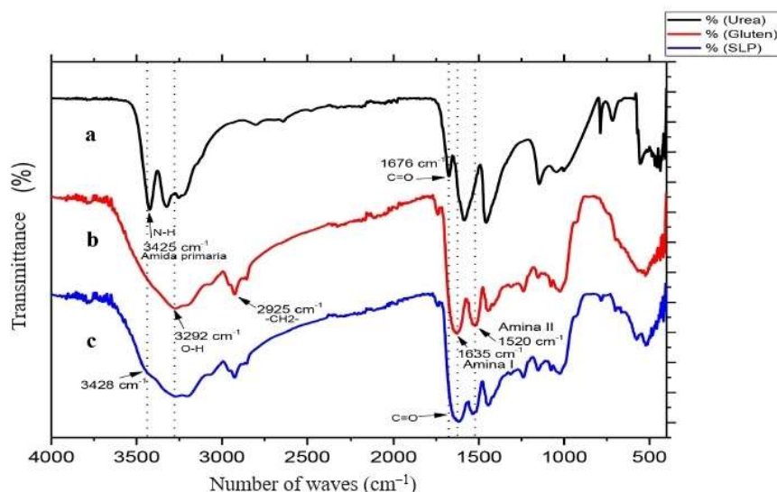
Figure 2. Analysis of the FT-IR spectra of the evaluated materials: (a) urea, (b) gluten powder, (c) SLIP powder.
