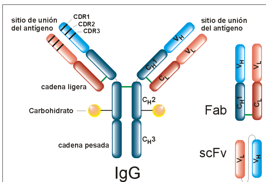
Figure 2. Structure of an IgG immunoglobulin and two of the most common fragments: the Fab fragment, obtained by enzymatic digestion of the antibody, and the scFv fragment, obtained by genetic engineering. Source: own elaboration.
