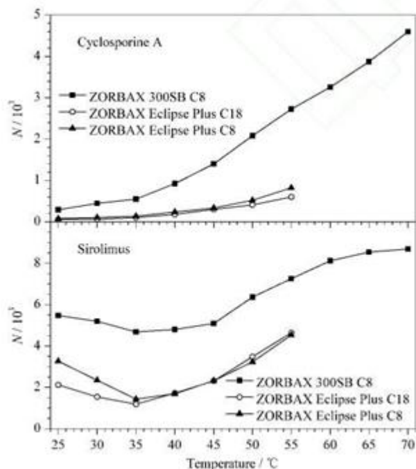
Figure 6. Relationships between the column temperature and chromatographic efficiency of cyclosporine A and sirolimus on different chromatography columns
