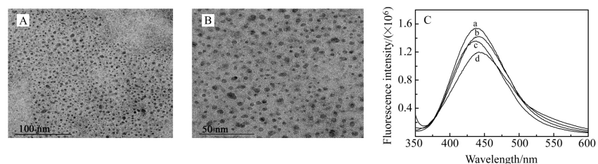
Figure 1 TEMI images of low (A) and high(B) magnification of GQDs ; fluorescence spectra of GQDs (C)(the excitation wavelength: a)320 nm, b)310 nm, c)330 nm and(d)340 nm)
