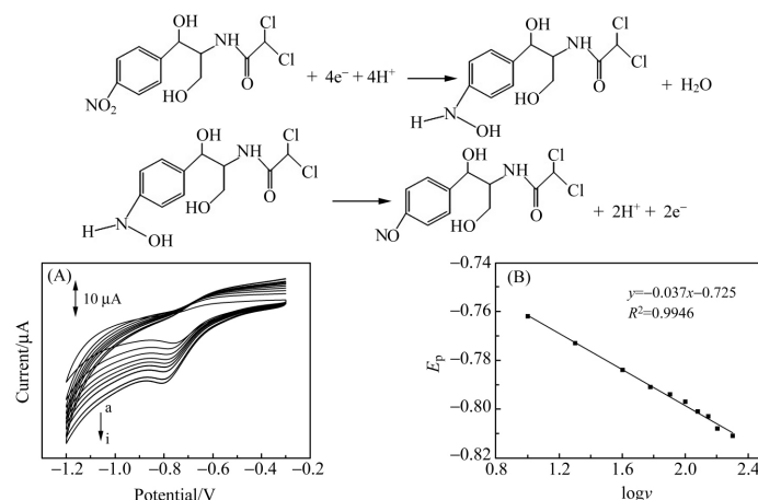
Figure 5 (A) Cyclic voltammograms of 1.0 \times 10^{-4} Mol/L CAP at the Nafion/GQDs/GCE (scan rates (a→i): 10, 40, 60, 80, 100, 120, 140, 160, 200 mV/s); (B) Linear plot of reduction potential vs. \log v
