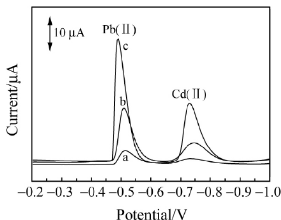
Figure 2 Anode stripping voltammograms of 2.40 \times 10^{-7} Mol/L Pb(II) and 9.80 \times 10^{-7} Mol/L Cd(II) at the bare GCE(a), Nafion/GCE(b) and Nafion/GQDs/GCE(c)
