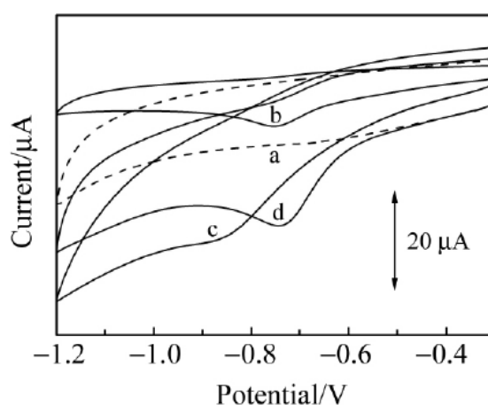
Figure 4 Cyclic voltammograms of 0mol/L(a) and 1.0 \times 10^{-4} Mol/L CAP in TE buffer solution(ph=7.0) at the bare GCE(b), Nafion/GCE(c) and Nafion/GQDs/GCE(a, d)
