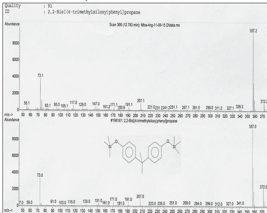
Figure 2. BPA: search and comparison with library spectrum.
