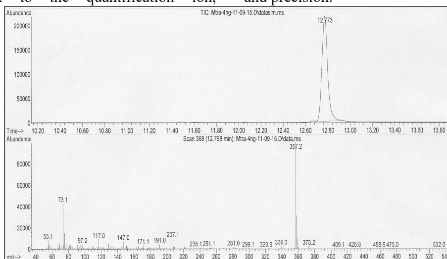
Figure 1. SIM chromatogram and mass spectrum of BPA.
