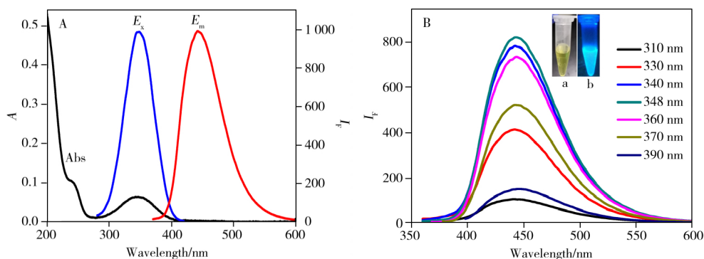
Figure 2 UV-Vis absorption spectrum and excitation/emission spectra of Cu-CDs(A) and fluorescence emission spectra with different excitation wavelengths(B) inset: photographs of Cu-CDs in aqueous solution under visible light(a) and UV light(b, 365 nm)
