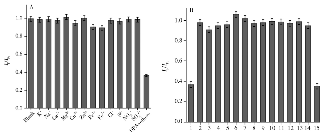
Figure 4 Selectivity of fluorescence system 1-15: zero point one five \mu\text{mol/L} DPA; six \mu\text{mol/L} of glucose, vitamin C, citric acid, sucrose, benzoic acid, phthalic acid, isophthalic acid, terephthalic acid, nicotinic acid, phenylalanine, cysteine, tryptophan, serine, the mixture of 0.15Mmol/L DPA with 6Mmol/L of different organic small molecules, respectively
