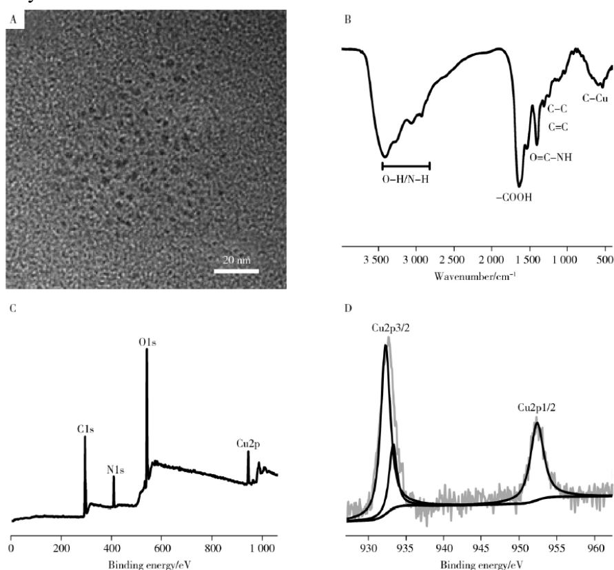
Figure 1 TEM image(A), FT-IR spectrum(B), XPS spectrum(C) of Cu-CDs and Cu2p high-resolution XPS spectrum(D)
