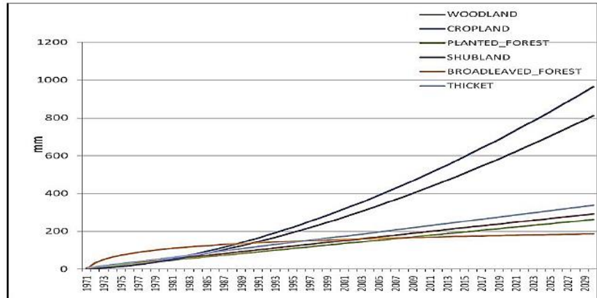
Figure 5. Expected JJAS runoff under specific effects of land cover change in Wundanyi by 2030 (1970 = 0) (Source: Data analysis by authors).
